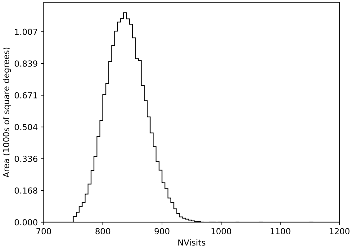
too_elab_r8_d3_griz_v3.4_10yrs WFD all bands: NVisits
