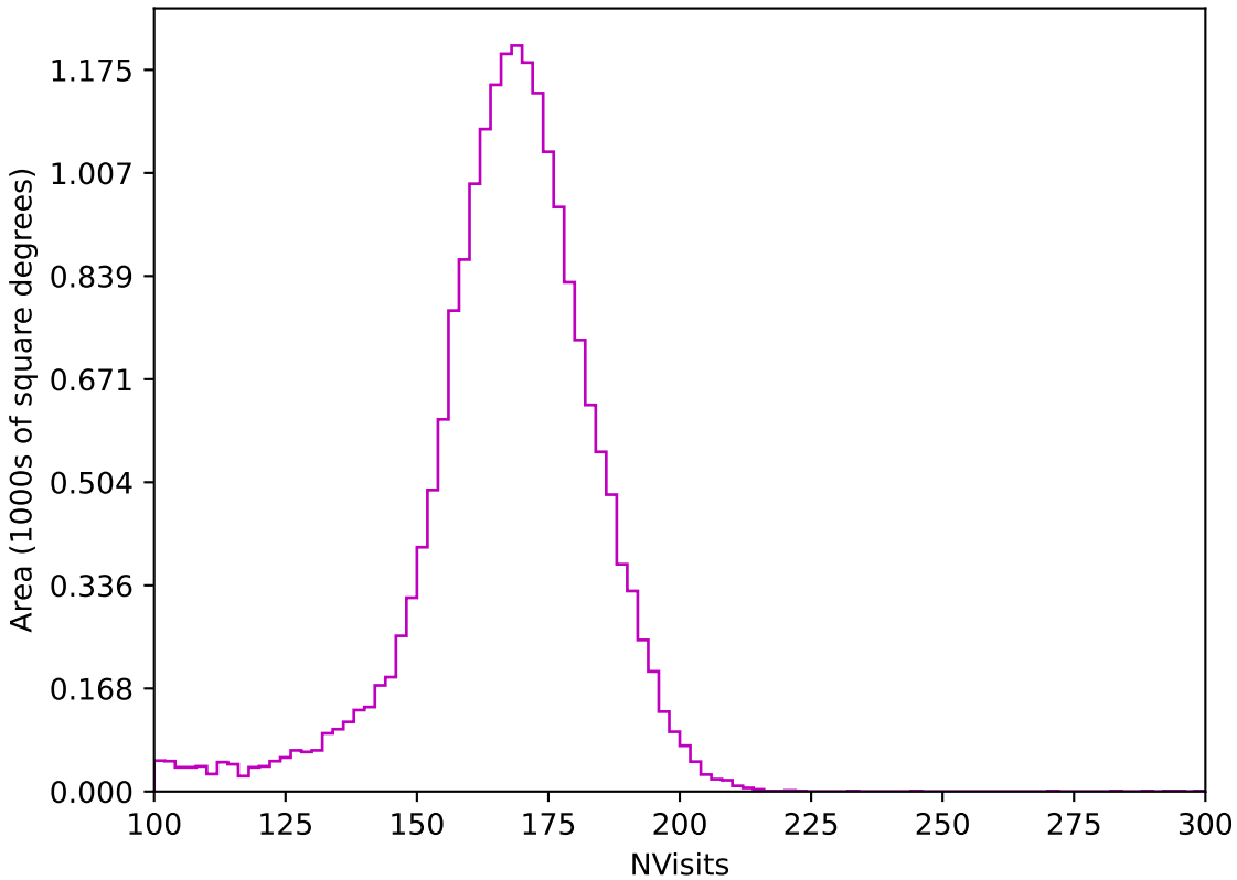
too_elab_r8_d3_griz_v3.4_10yrs All sky z band: NVisits
