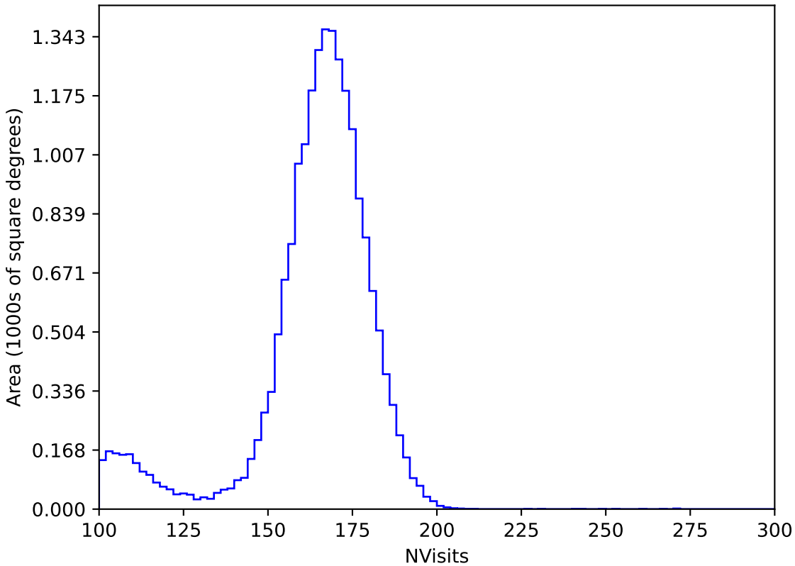
too_elab_r8_d3_griz_v3.4_10yrs All sky y band: NVisits
