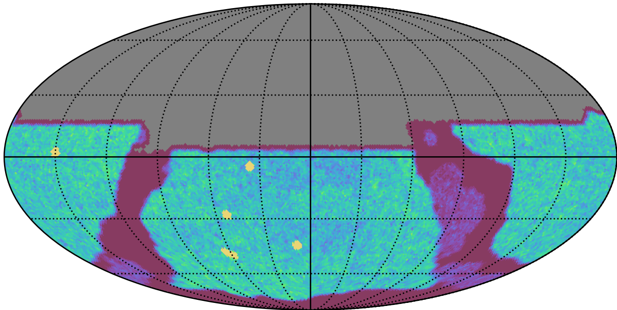
too_elab_r8_d3_griz_v3.4_10yrs All sky u band: NVisits
