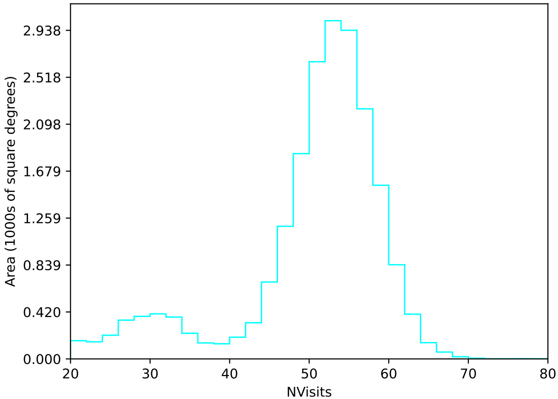
too_elab_r8_d3_griz_v3.4_10yrs All sky u band: NVisits
