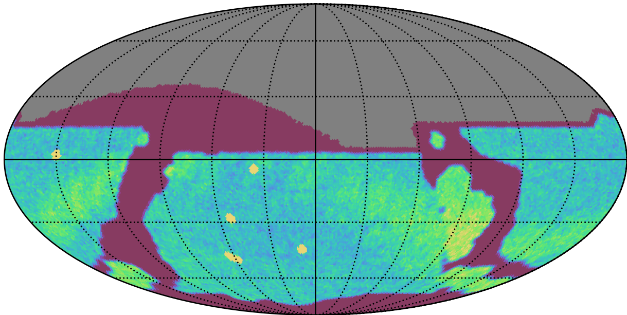
too_elab_r8_d3_griz_v3.4_10yrs All sky r band: NVisits
