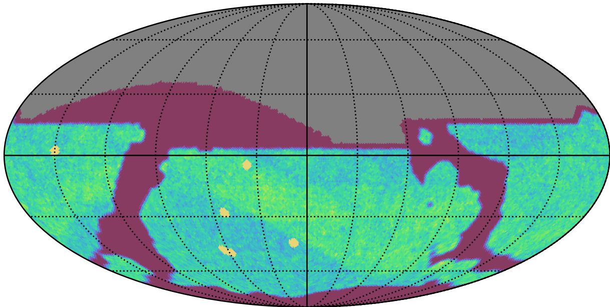
too_elab_r8_d3_griz_v3.4_10yrs All sky i band: NVisits
