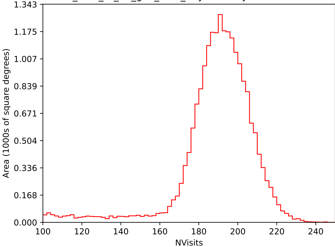
too_elab_r8_d3_griz_v3.4_10yrs All sky i band: NVisits
