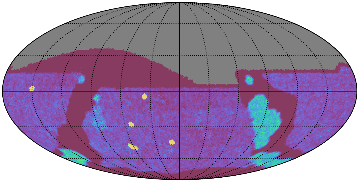
too_elab_r8_d3_griz_v3.4_10yrs All sky g band: NVisits
