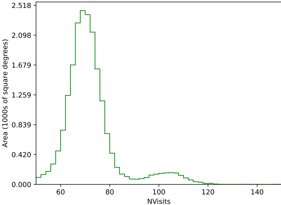
too_elab_r8_d3_griz_v3.4_10yrs All sky g band: NVisits
