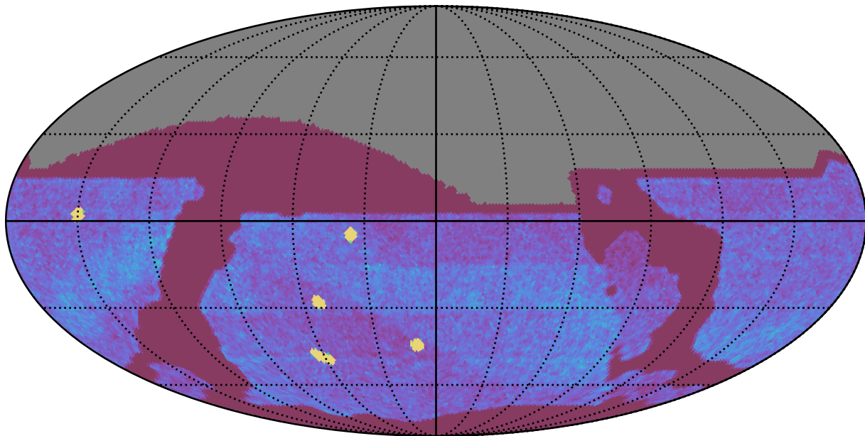
too_elab_r8_d3_griz_v3.4_10yrs All sky all bands: NVisits
