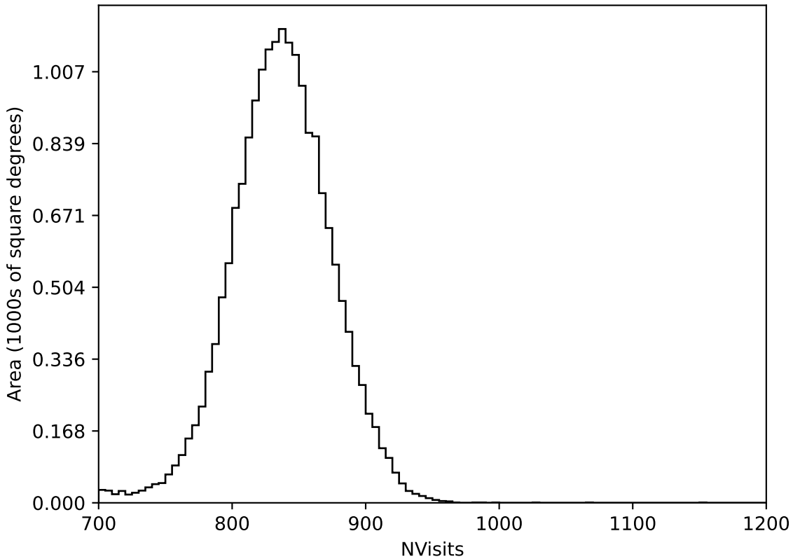
too_elab_r8_d3_griz_v3.4_10yrs All sky all bands: NVisits
