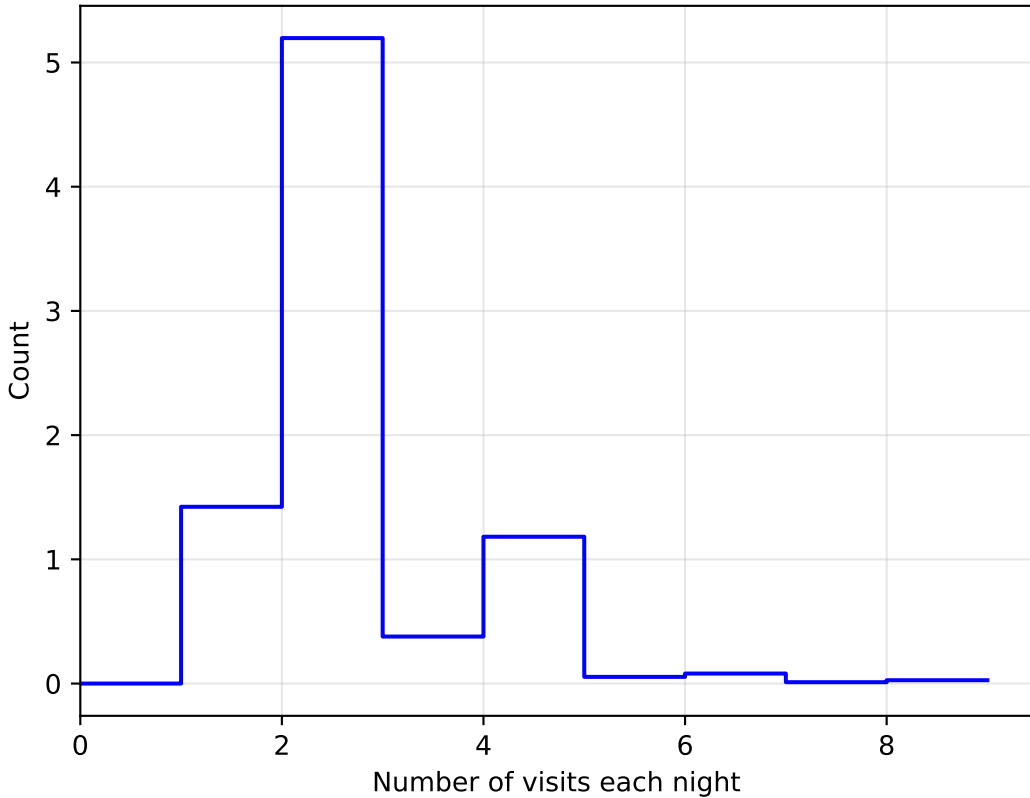
too_elab_r8_d3_griz_v3.4_10yrs WFD: NVisitsPerNight
