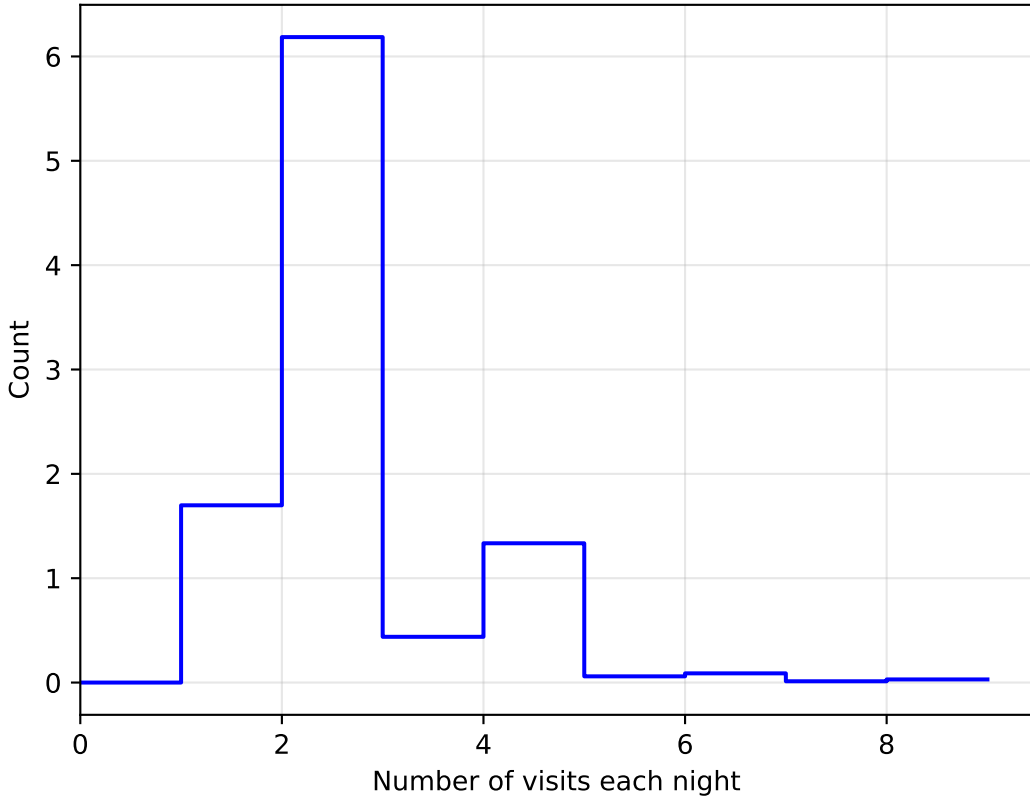
too_elab_r8_d3_griz_v3.4_10yrs All sky: NVisitsPerNight
