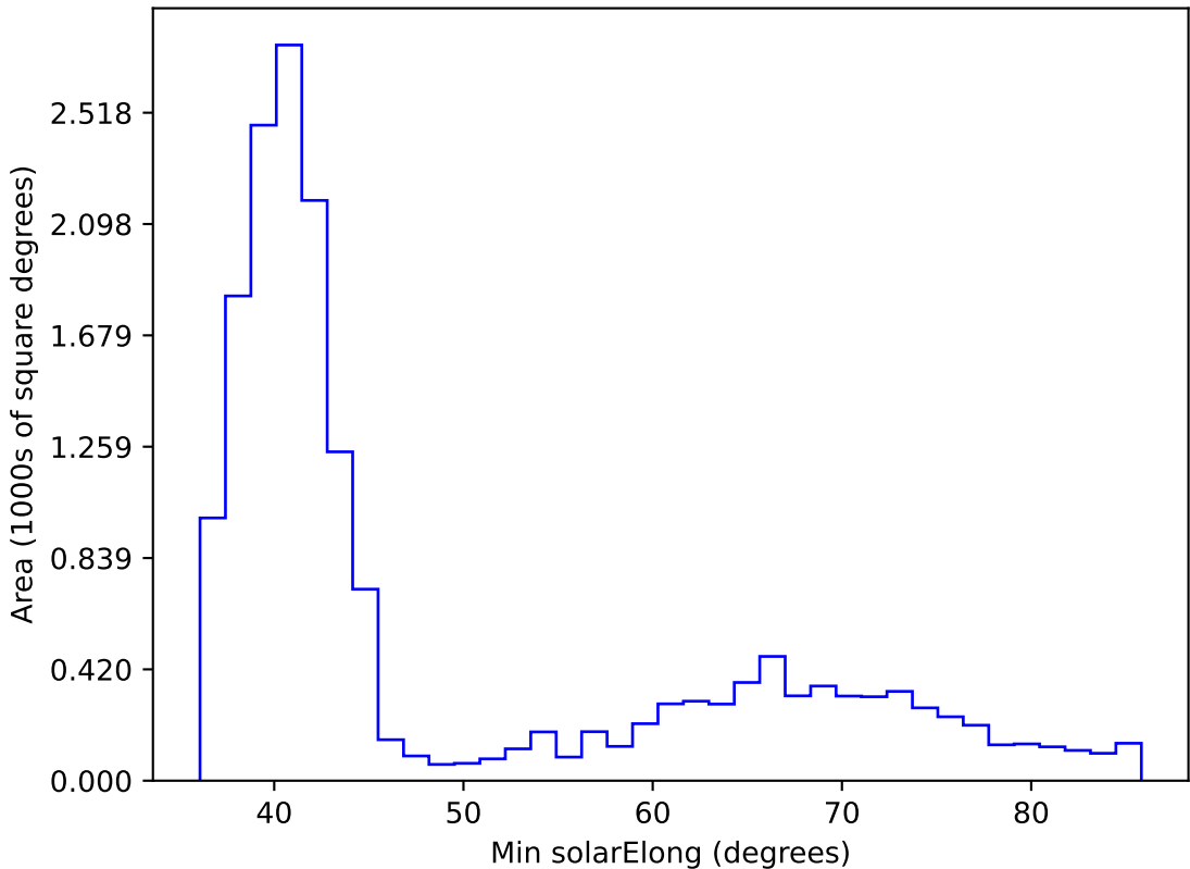
too_elab_r8_d3_griz_v3.4_10yrs WFD z band: Min solarElong
