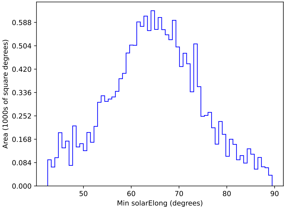
too_elab_r8_d3_griz_v3.4_10yrs WFD y band: Min solarElong
