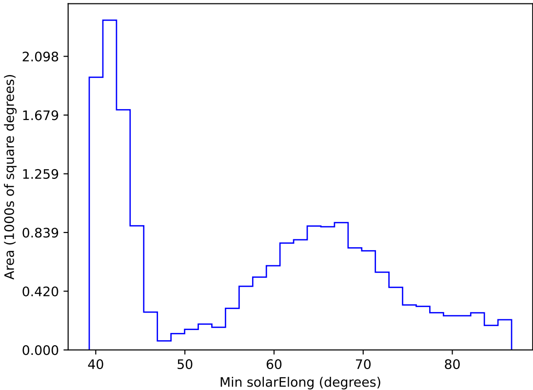
too_elab_r8_d3_griz_v3.4_10yrs WFD r band: Min solarElong
