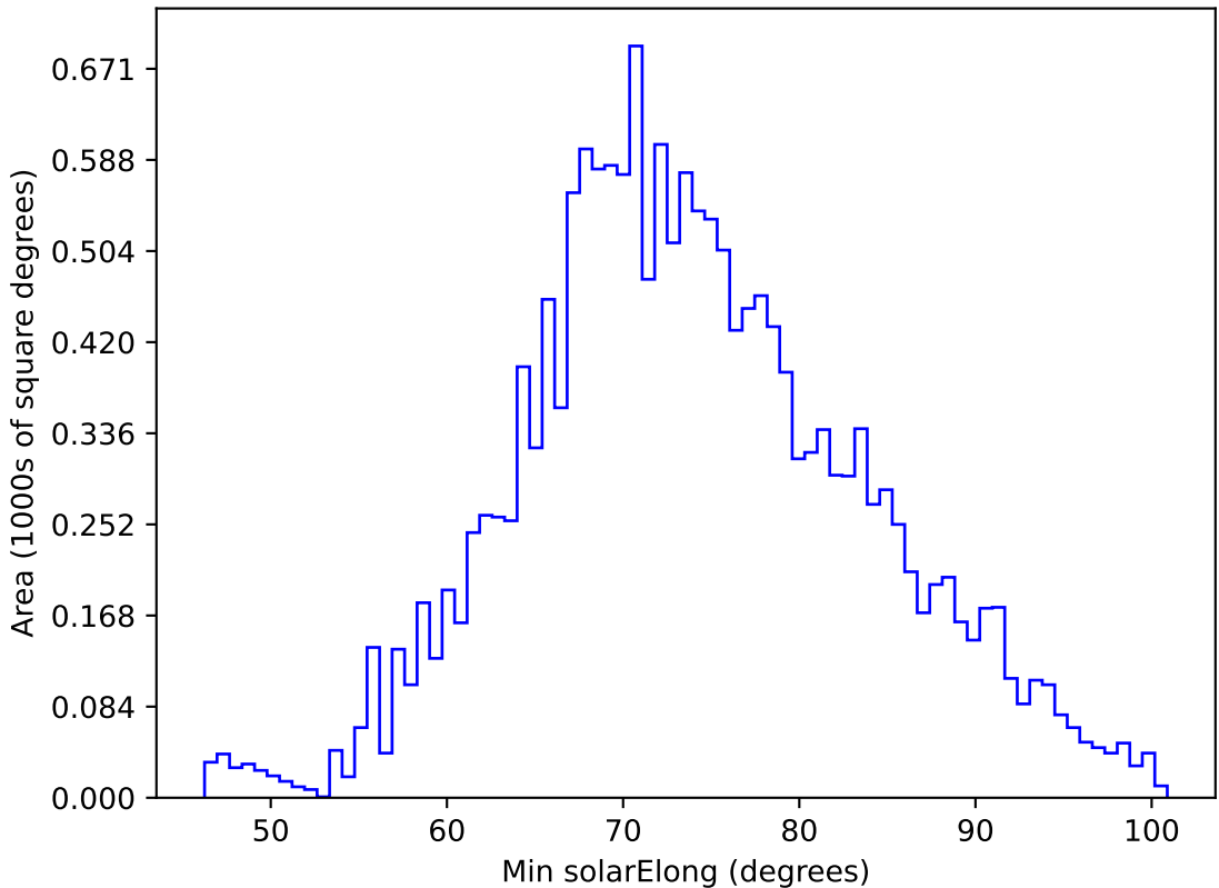
too_elab_r8_d3_griz_v3.4_10yrs WFD g band: Min solarElong
