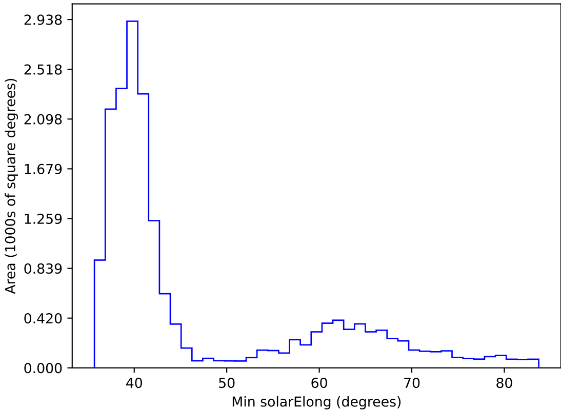
too_elab_r8_d3_griz_v3.4_10yrs WFD all bands: Min solarElong
