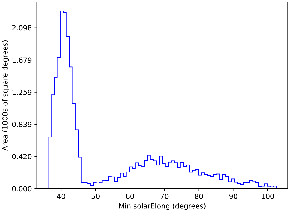
too_elab_r8_d3_griz_v3.4_10yrs All sky z band: Min solarElong
