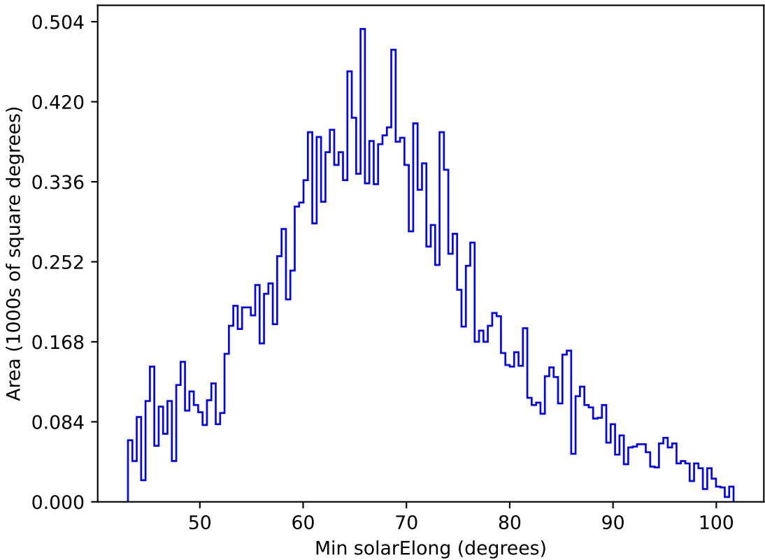
too_elab_r8_d3_griz_v3.4_10yrs All sky y band: Min solarElong
