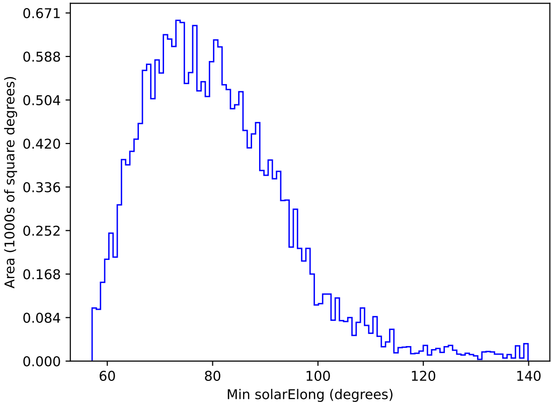
too_elab_r8_d3_griz_v3.4_10yrs All sky u band: Min solarElong
