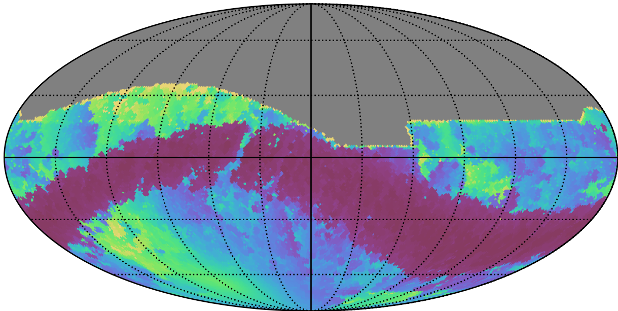
too_elab_r8_d3_griz_v3.4_10yrs All sky r band: Min solarElong
