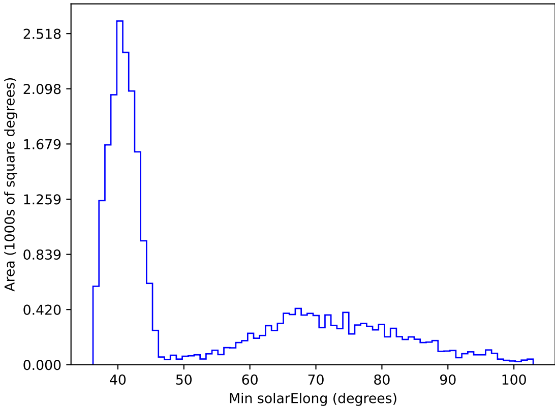
too_elab_r8_d3_griz_v3.4_10yrs All sky i band: Min solarElong
