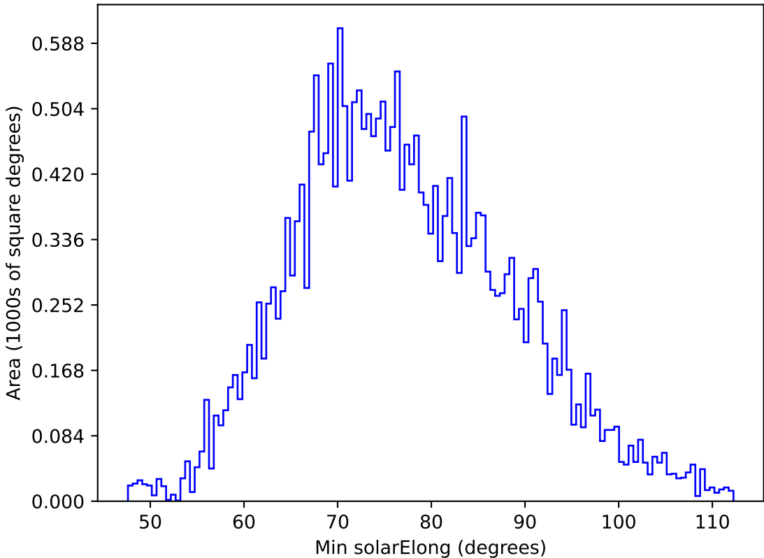
too_elab_r8_d3_griz_v3.4_10yrs All sky g band: Min solarElong
