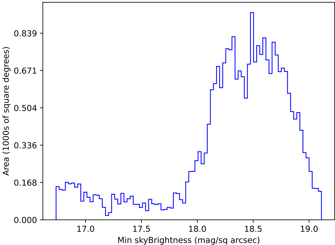
too_elab_r8_d3_griz_v3.4_10yrs Yr 1 z band: Min skyBrightness
