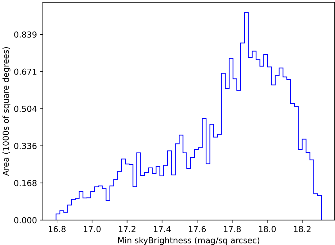
too_elab_r8_d3_griz_v3.4_10yrs Yr 1 y band: Min skyBrightness
