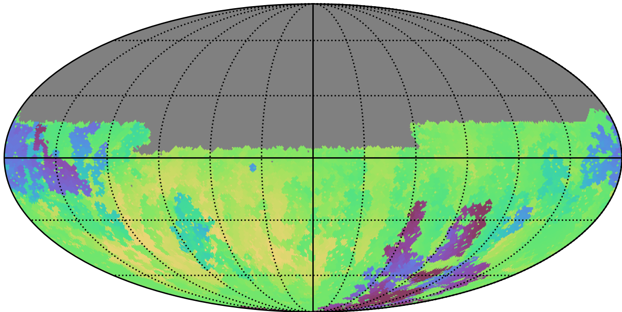
too_elab_r8_d3_griz_v3.4_10yrs Yr 1 u band: Min skyBrightness
