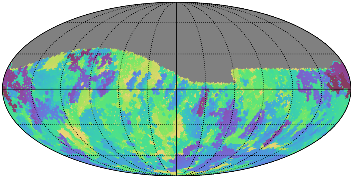
too_elab_r8_d3_griz_v3.4_10yrs Yr 1 r band: Min skyBrightness
