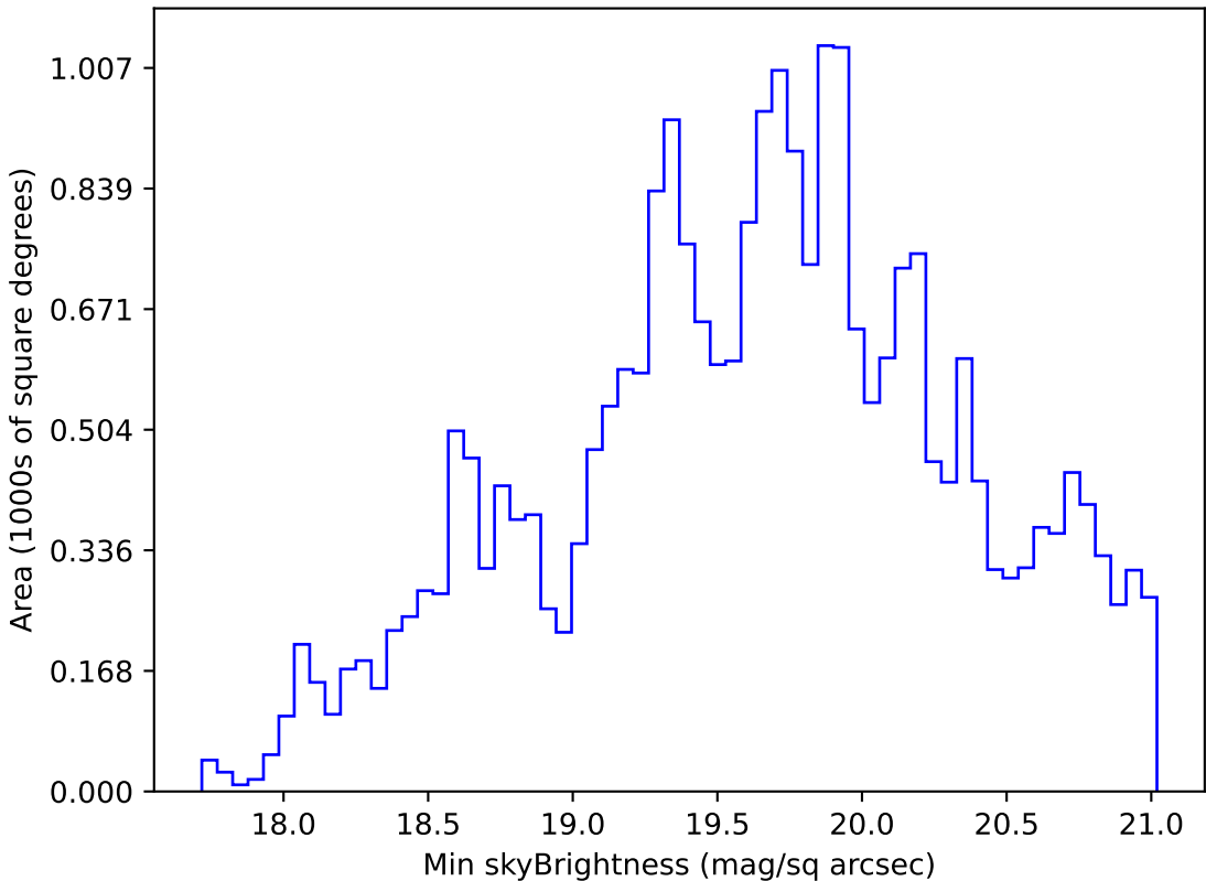
too_elab_r8_d3_griz_v3.4_10yrs Yr 1 r band: Min skyBrightness
