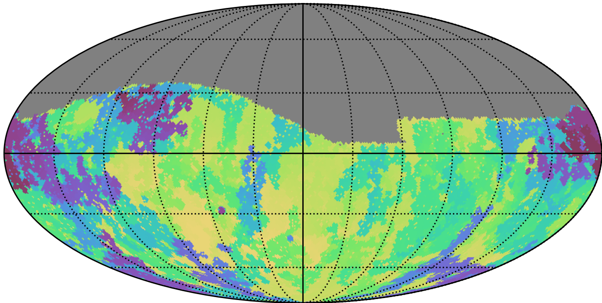
too_elab_r8_d3_griz_v3.4_10yrs Yr 1 g band: Min skyBrightness
