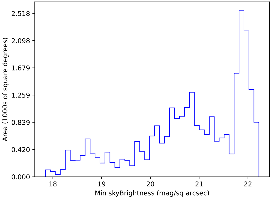
too_elab_r8_d3_griz_v3.4_10yrs Yr 1 g band: Min skyBrightness
