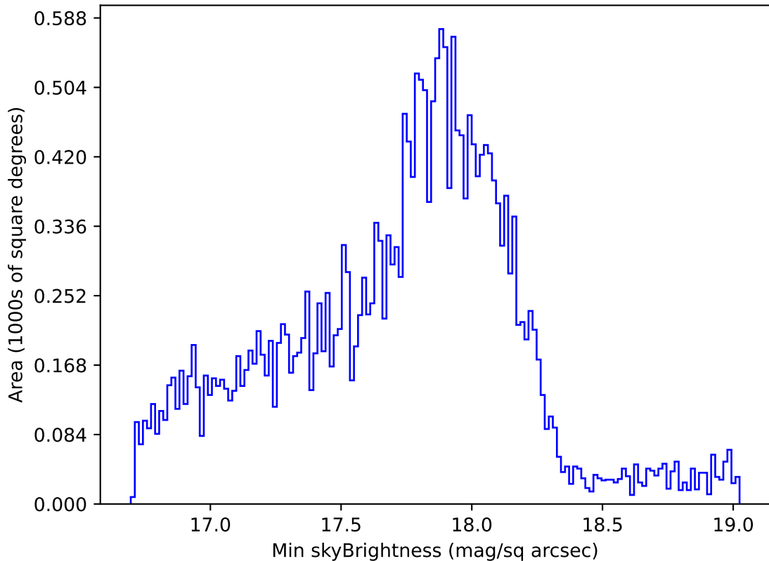
too_elab_r8_d3_griz_v3.4_10yrs Yr 1 all bands: Min skyBrightness
