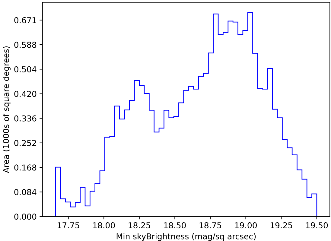
too_elab_r8_d3_griz_v3.4_10yrs WFD r band: Min skyBrightness
