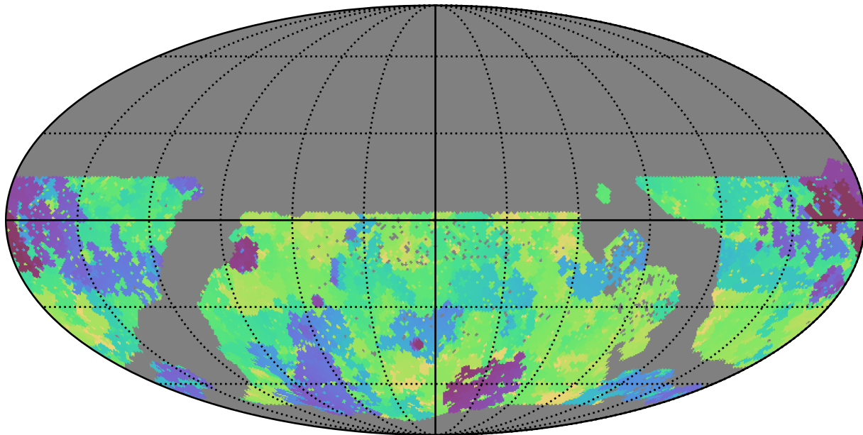
too_elab_r8_d3_griz_v3.4_10yrs WFD g band: Min skyBrightness
