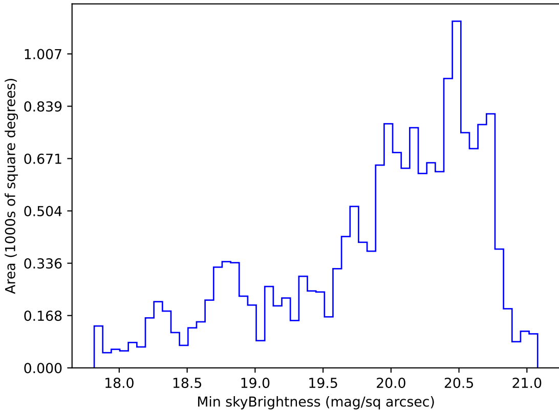
too_elab_r8_d3_griz_v3.4_10yrs WFD g band: Min skyBrightness
