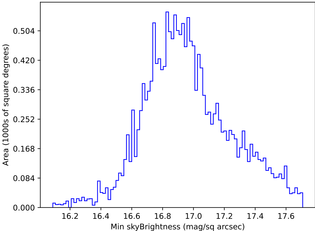
too_elab_r8_d3_griz_v3.4_10yrs WFD all bands: Min skyBrightness
