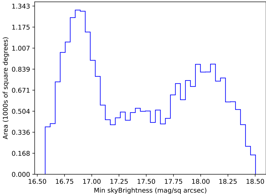
too_elab_r8_d3_griz_v3.4_10yrs All sky z band: Min skyBrightness
