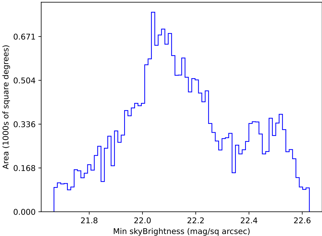
too_elab_r8_d3_griz_v3.4_10yrs All sky u band: Min skyBrightness
