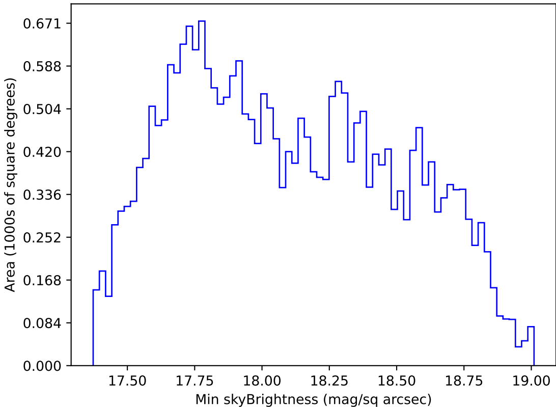
too_elab_r8_d3_griz_v3.4_10yrs All sky i band: Min skyBrightness
