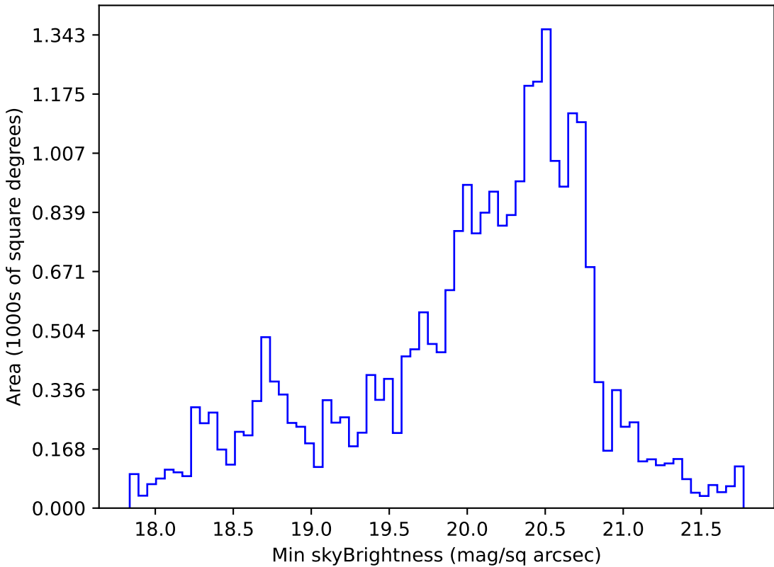
too_elab_r8_d3_griz_v3.4_10yrs All sky g band: Min skyBrightness
