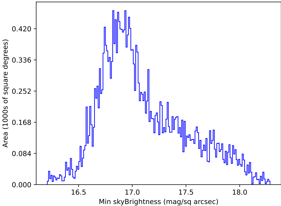
too_elab_r8_d3_griz_v3.4_10yrs All sky all bands: Min skyBrightness
