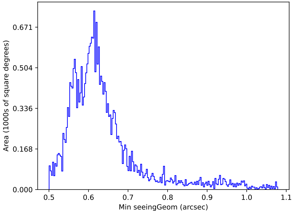
too_elab_r8_d3_griz_v3.4_10yrs Yr 1 r band: Min seeingGeom
