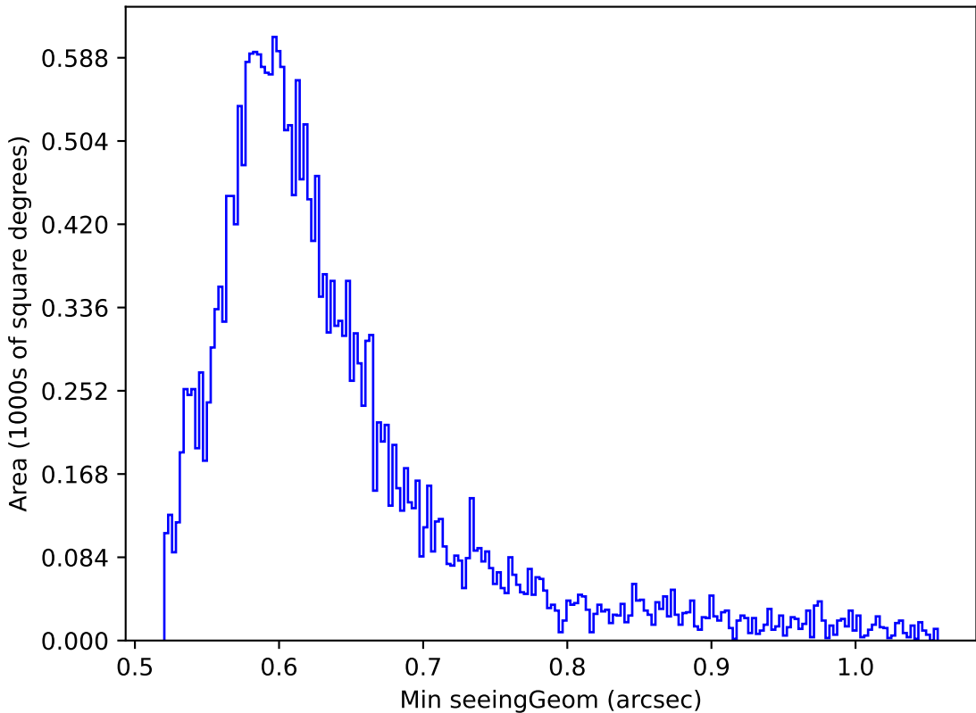
too_elab_r8_d3_griz_v3.4_10yrs Yr 1 i band: Min seeingGeom
