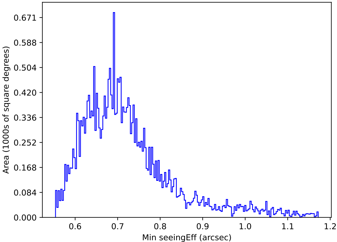
too_elab_r8_d3_griz_v3.4_10yrs Yr 1 z band: Min seeingEff
