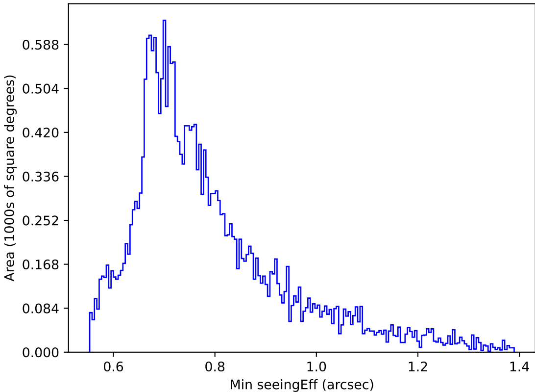
too_elab_r8_d3_griz_v3.4_10yrs Yr 1 g band: Min seeingEff
