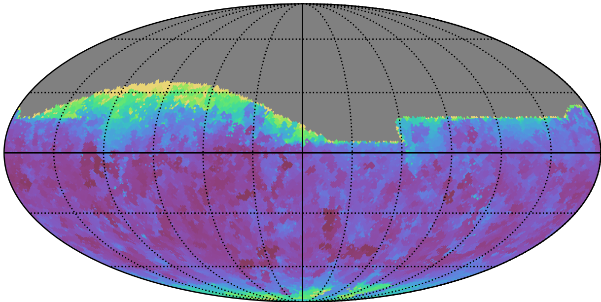
too_elab_r8_d3_griz_v3.4_10yrs Yr 1 all bands: Min seeingEff
