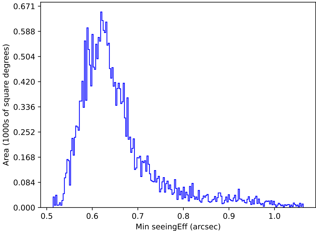
too_elab_r8_d3_griz_v3.4_10yrs Yr 1 all bands: Min seeingEff
