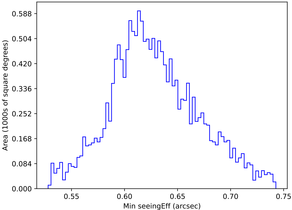
too_elab_r8_d3_griz_v3.4_10yrs WFD y band: Min seeingEff
