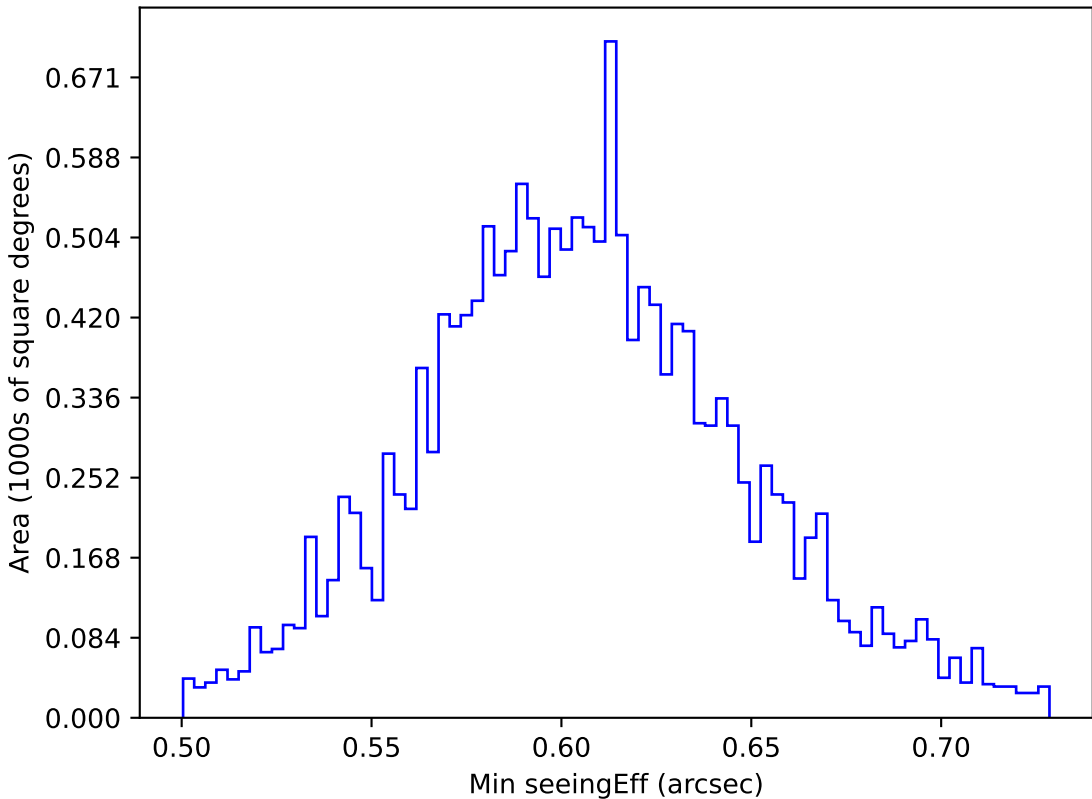
too_elab_r8_d3_griz_v3.4_10yrs WFD i band: Min seeingEff
